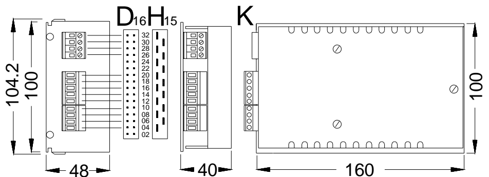
open-frame front and top views
