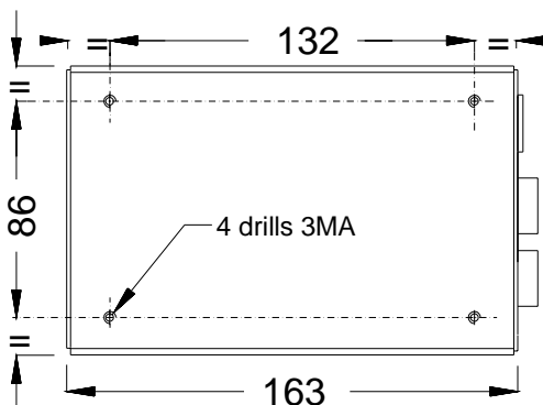
enclosure -C- side and top views
